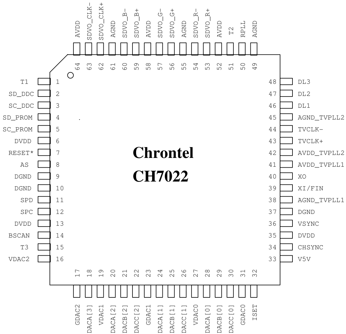
Figure 2: 64-Pin LQFP Package
